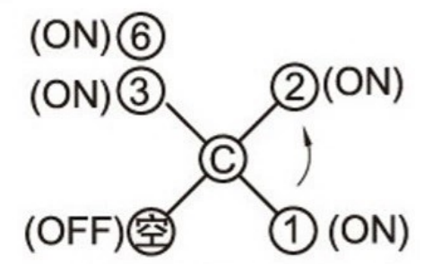
SCHEMATIC (NON-SHORTING)
